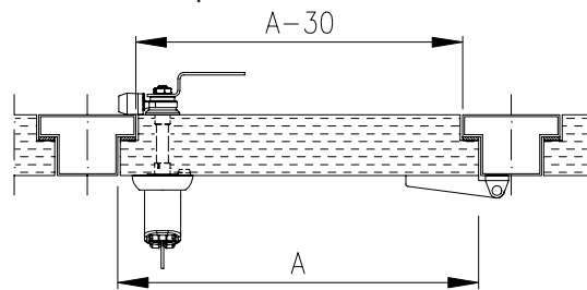
Inward opening inspection door for LQTC
