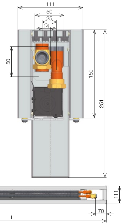
The given dimensions are in mm.
