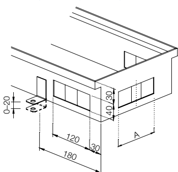
The sketches dimensions are given in mm.
