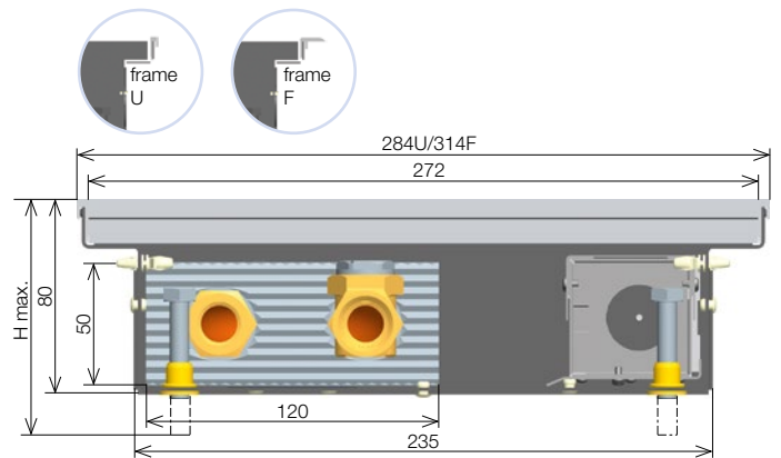
The given dimensions are in mm and with the frames U and F.
