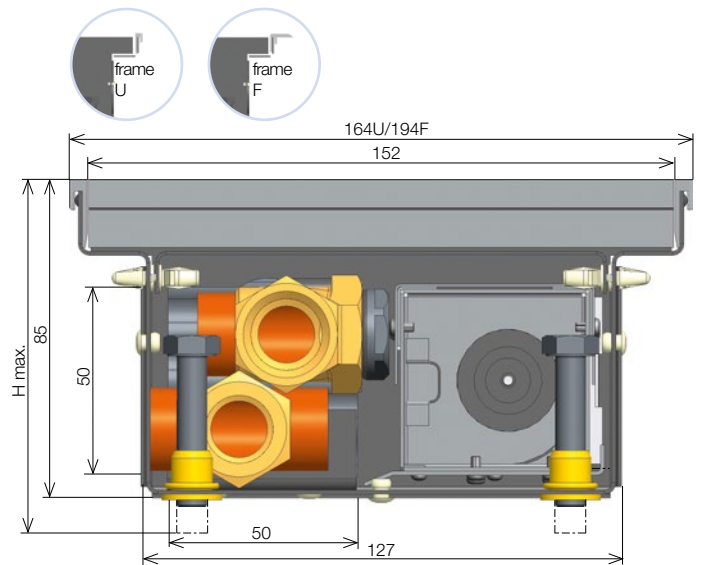
The given dimensions are in mm and with the frames U and F.
