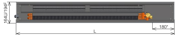
The given dimensions are in mm and with the frames U and F.
